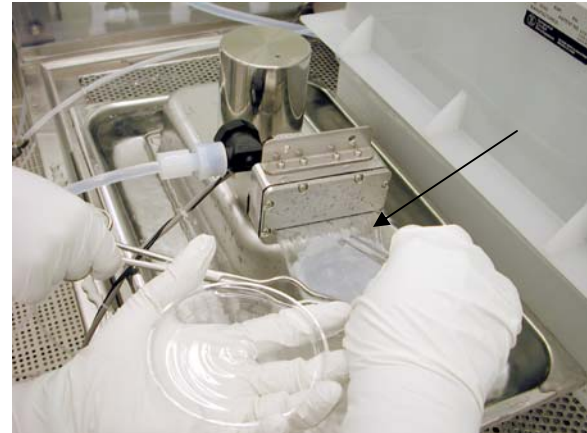
Figure 1: UPW/Megasonic cleaning set-up for small fragments. Fragment (arrow) is gripped with tweezers only on edge and held in flowing stream for 5 minutes.
